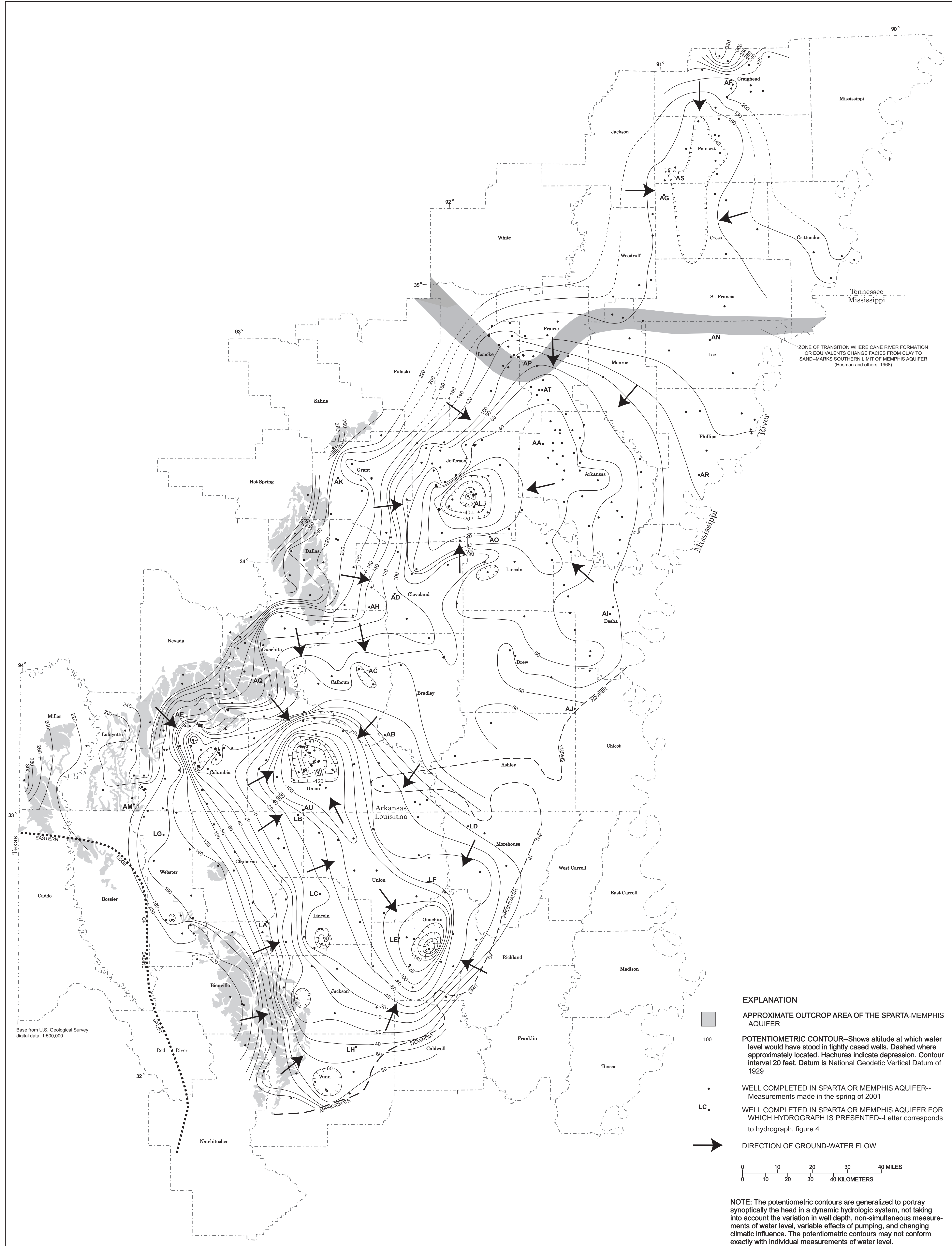
POTENTIOMETRIC SURFACE OF THE SPARTA-MEMPHIS AQUIFER IN ARKANSAS AND LOUISIANA, SPRING 2001 T.P. Schrader 2004
