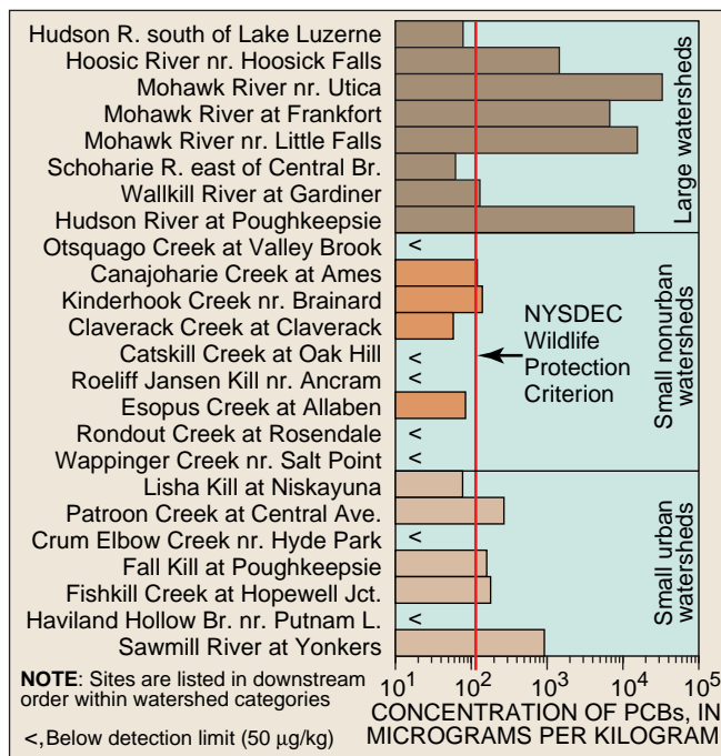
Figure 6. Concentrations of PCBs in whole carp or white suckers from 24 sites in the Hudson River Basin. Concentrations were highest and often exceeded the Wildlife Protection Criterion in large rivers and some urban streams.
