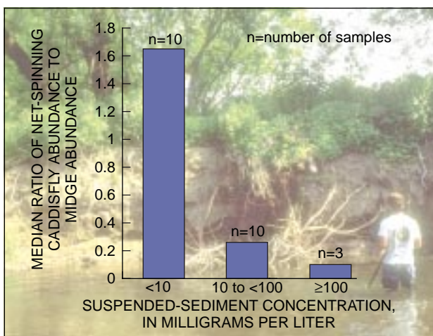
Figure 9. Median ratio of net-spinning caddisfly abundance to midge abundance as it relates to suspended-sediment concentration during high flows. Exposed streambanks, like that pictured above, are common in agricultural and urban areas; these banks are susceptible to erosion, and they supply higher than normal amounts of sediment to streams.
