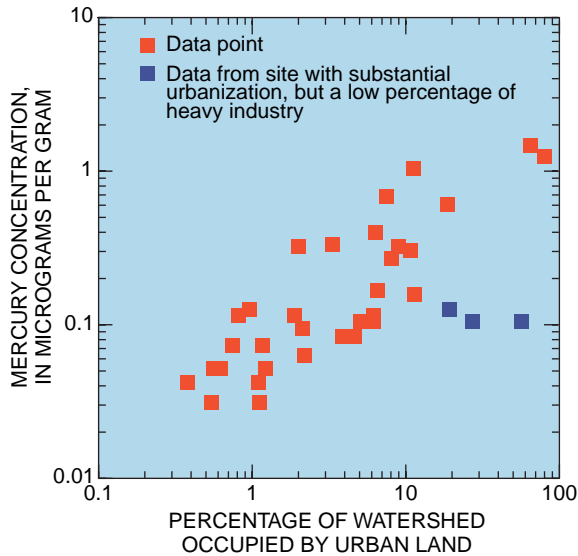
Figure 2. Mercury concentration in stream-bottom sediment in relation to the percentage of urban land in watersheds of the Hudson River Basin. Streams draining urban areas generally had higher concentrations of mercury in stream-bottom sediments than nonurban and urban watersheds without heavy industry.
