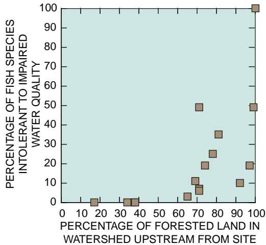
Figure 8. Percentage of intolerant fish species at a site as a function of the amount of forested land within the watershed. The absence or rarity of fish intolerant to impaired water quality was associated with chemical and (or) habitat impairment more often found in developed watersheds than in forested watersheds.
