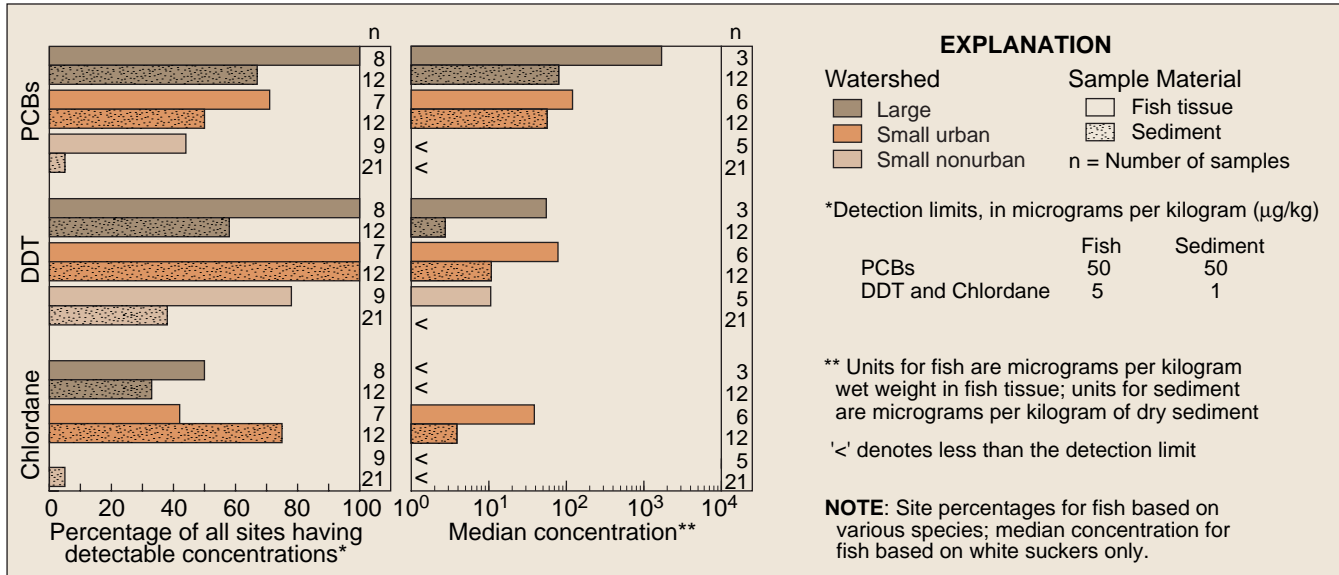
Figure 4. Detection of PCBs, DDT compounds, and chlordane compounds in fish tissue and stream-bottom sediments in Hudson River Basin watersheds. These compounds were generally detected more often and at higher concentrations in fish tissue than stream-bottom sediments.
