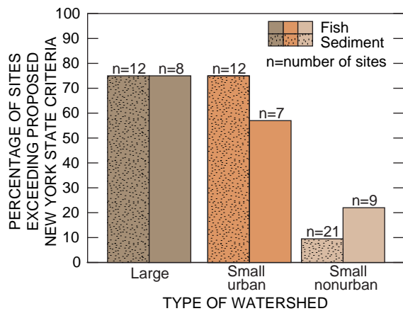
Figure 5. Percentage of sites at which proposed NYSDEC screening criteria for at least one organochlorine compound in fish tissue and stream-bottom sediment were exceeded. Large and small urban watersheds regularly exceeded these criteria in fish-tissue and stream-bottom sediment.
