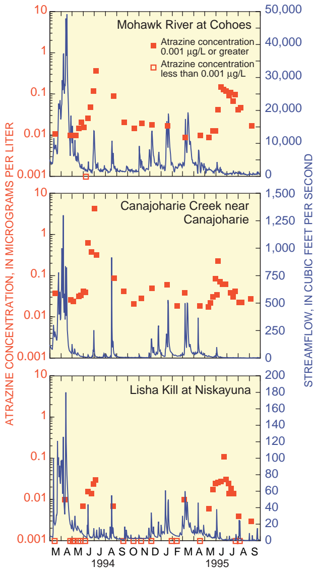
Figure 12. Atrazine concentration and streamflow at the three fixed sites (locations are shown in fig. 11). The highest concentration of atrazine and other pesticides generally occurred during the first runoff after pesticide application.
