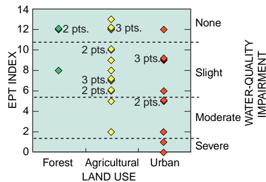
Figure 7. Invertebrate-community survey results from a USGS sampling of 28 streams in the Hudson River Basin. Most streams sampled show some impairment. Severe water-quality impairment was observed at sites in the most highly developed urban watersheds.
