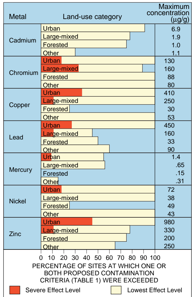
Figure 1. Percentage of sites at which one or both New York State proposed screening criteria for metals contamination in stream-bottom sediment were exceeded, and maximum concentrations of metals by land-use category. Sites in urban and large-mixed watersheds had the highest concentrations and often exceeded both criteria.
