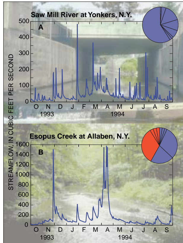
Figure 10. Streamflow and abundance of fish for: (A) “flashy” (sharply changing) streamflow that results from urbanization and (B) streamflow more typical of undisturbed conditions. Pie charts represent the fish community at each site. Number of slices indicates the number of species observed; size of slice represents the number of individuals in relation to the other species present. Blue indicates species tolerance to impaired water quality; red indicates intolerance. Channelized conditions and associated flashy streamflow likely contributed to the unbalanced fish community observed at the Saw Mill River and similar sites.
