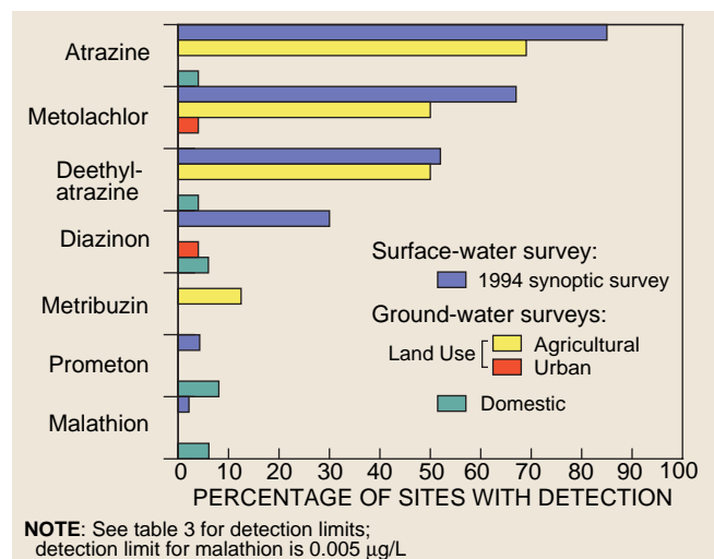
Figure 13. Detection of seven selected pesticides in three ground-water surveys and in a 1994 synoptic survey of streams throughout the Hudson River Basin. Among the ground-water surveys, pesticides were most often detected in shallow ground water beneath agricultural areas, but detection percentages in streams were generally highest.
