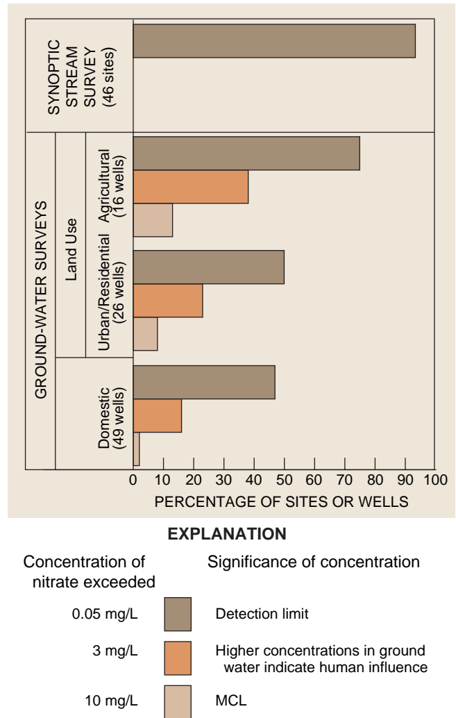
Figure 14. Percentage of nitrate concentrations in wells and 1993 synoptic stream-sampling sites that exceeded the indicated concentrations. Nitrate was most often detected in a synoptic survey of surface water, but never at concentrations greater than 1.4 mg/L. The highest concentrations were in ground water from beneath agricultural fields.
