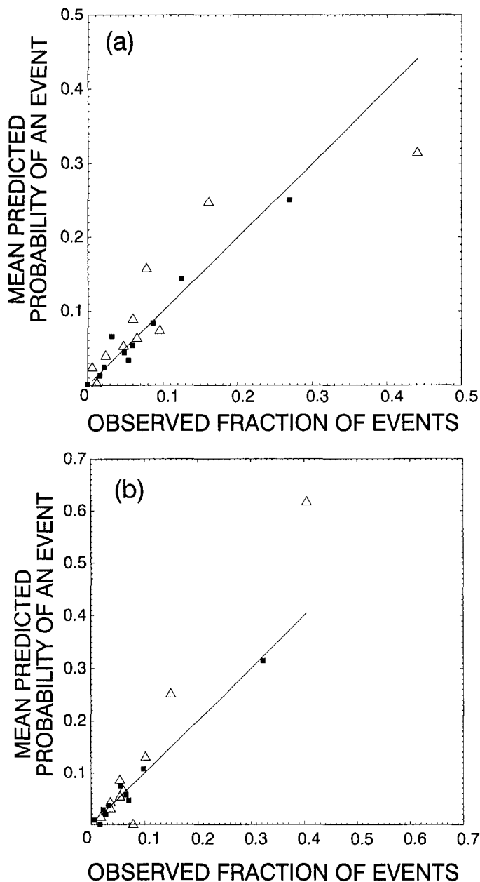
Fig. 6. The average predicted fraction of wells with nitrate concentrations \geq 3 mg/l vs. observed for each decile of risk: aquifer susceptibility model (6a) and ground-water vulnerability model (6b). Boxes and triangles display WDOH and NWIS data respectively. Predicted = observed lines are also shown.
