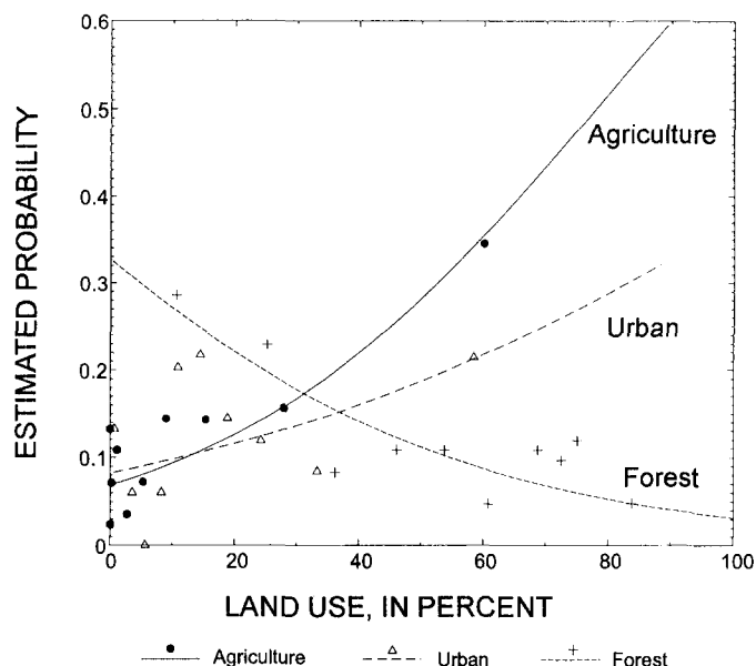
Fig. 4. Lines depict the estimated probability of encountering nitrate concentrations \geq 3 mg/l as a function of percentage land use within a 3.2-kilometer radius of the well. Data points represent the fraction of WDOH wells that have nitrate concentrations \geq 3 mg/l vs. mean land use for each decile of risk. Pluses, triangles, and circles are the data for forest, urban, and agricultural land uses, respectively.
