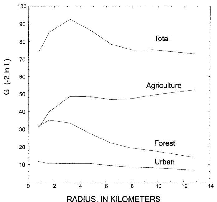
Fig. 3. G values vs. radius surrounding the WDOH wells used to calculate percent land use. Total was calculated by summing the three land-use types.
