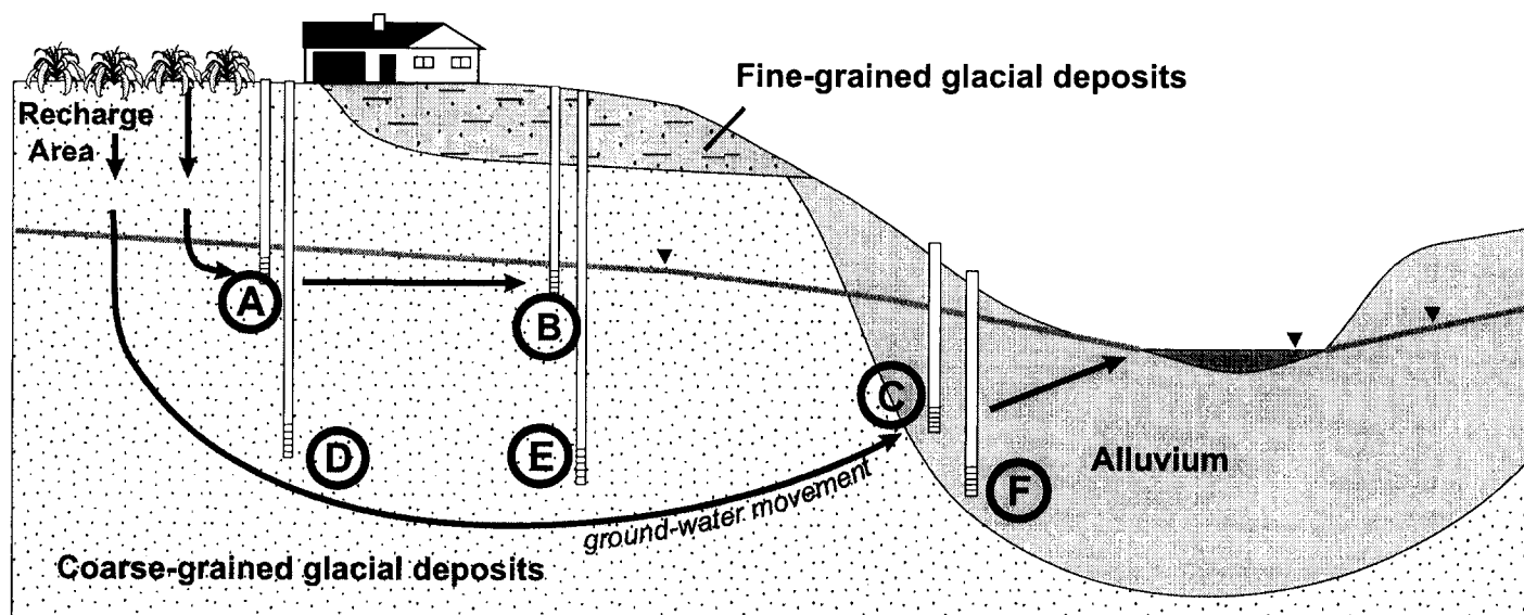
Fig. 7. Generalized cross section for an alluvial valley in the Puget Sound Basin (adapted from Vaccaro et al., 1997). Letters are points along flow paths as described in the text.
