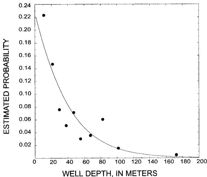
Fig. 2. The line depicts the estimated probability that nitrate concentrations in ground water are \geq 3 mg/l as a function of well depth for the WDOH data set. Data points show the fraction of wells which have nitrate concentrations \geq 3 mg/l vs. mean well depth for each decile of risk.
