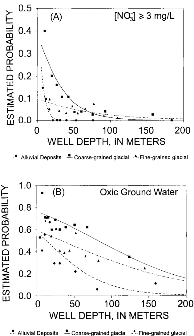
Fig. 5. (A) Lines depict the estimated probability that nitrate concentrations are \geq 3 mg/l vs. well depth for each surficial geology type. Data points show the fraction of WDOH wells that have nitrate \geq 3 mg/l vs. mean well depth for each decile of risk. (B) Lines depict estimated probability that dissolved oxygen concentrations are 1 mg/l in the NWIS data set. Data points represent the fraction of NWIS wells that have dissolved oxygen concentrations \geq 1 mg/l vs. mean well depth for each decile of risk.
