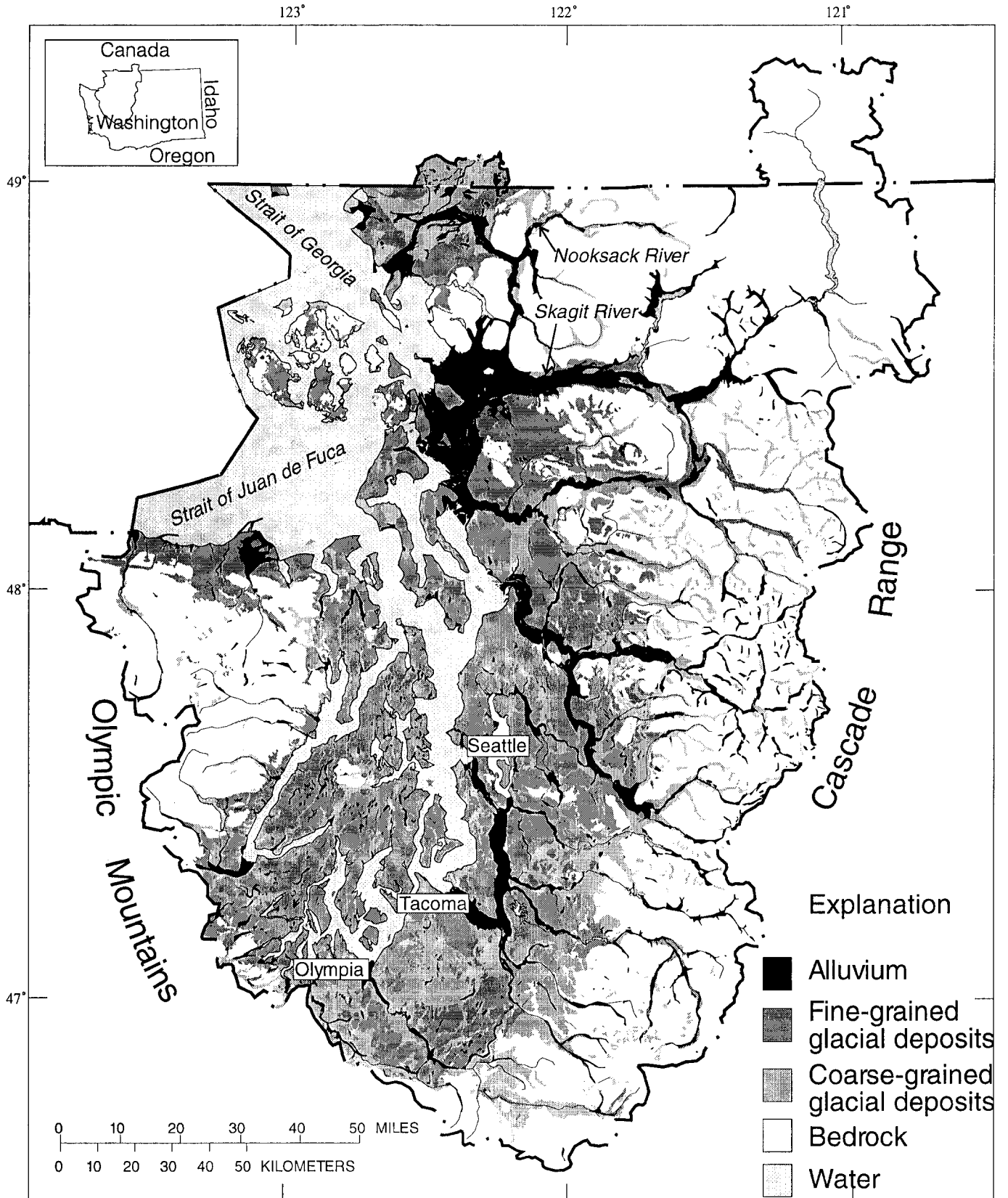
Fig. 1. Generalized surficial geology of the Puget Sound Basin (adapted from Jones, 1997).
