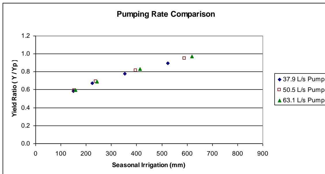
Figure 10. Example of the effects of various pumping rates. St. John, KS, 125 mm/m WHC, all years, recommended irrigation strategies.
