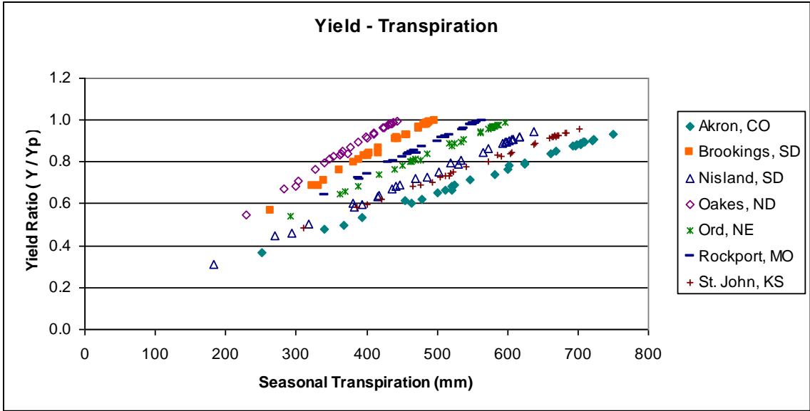
Figure 3. Yield-transpiration relationship for each site. Each point represents an irrigation strategy. Data is averaged across all WHCs, pumping rates, and years.
