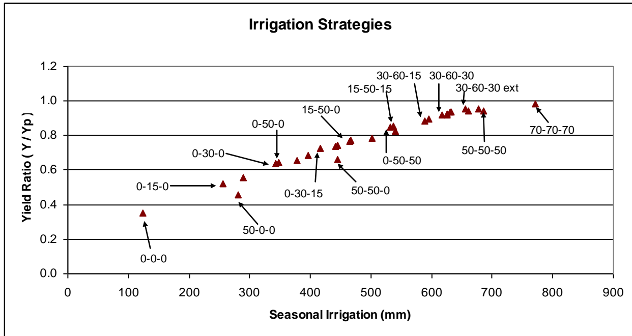
Figure 7. Example of yield-irrigation relationship with selected strategies labeled. Nisland, SD, all years, 83 mm/m WHC, 63.1 L/s pumping rate.
